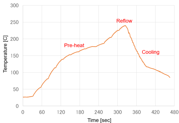
Figure 24. Example of a Reflow Profile
