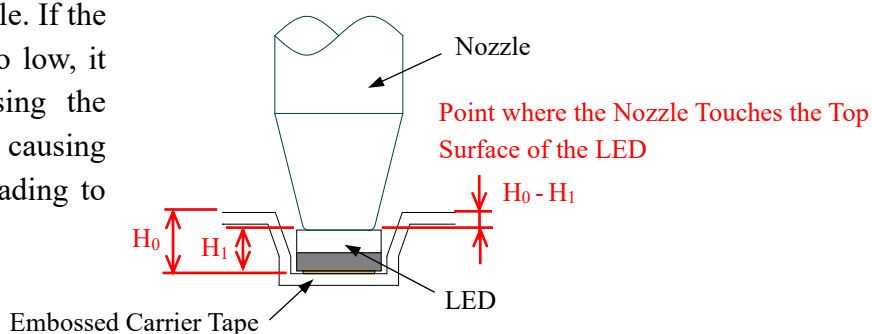
Figure 15. Recommended Nozzle Height for Pick-up Operation
