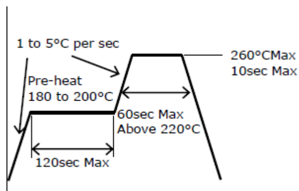
Figure 23. Reflow Soldering Condition (Lead-free Solder)
