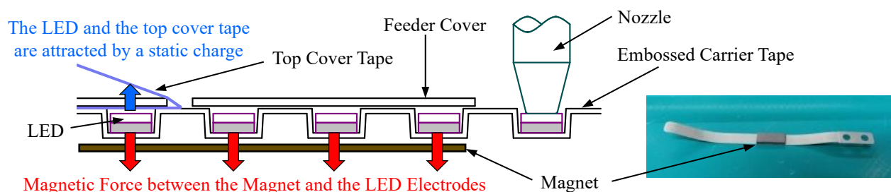
Figure 21. Magnet under the Embossed Carrier Tape
