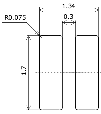
Figure 7. Soldering Pad Pattern and Metal Solder Stencil Aperture Pattern Recommended for the NCSx170x
