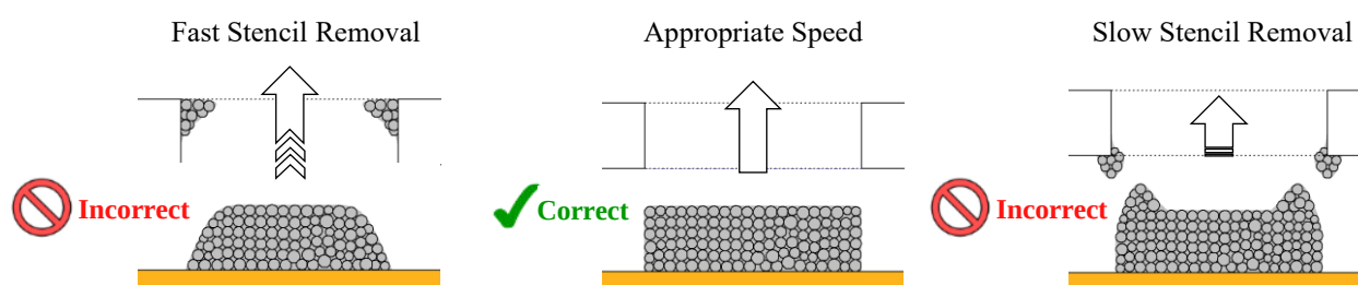
Figure 9. Speed of Solder Stencil Removal and Shape of the Solder Paste
