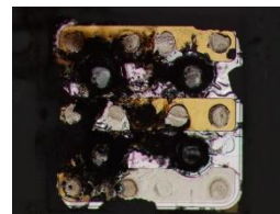
Damaged Electrodes of the LED chip due to an Inrush Current.
