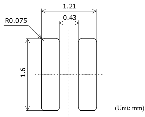
Figure 7. Soldering Pad Pattern and Metal Solder Stencil Aperture Pattern Recommended for the NCSx170x
