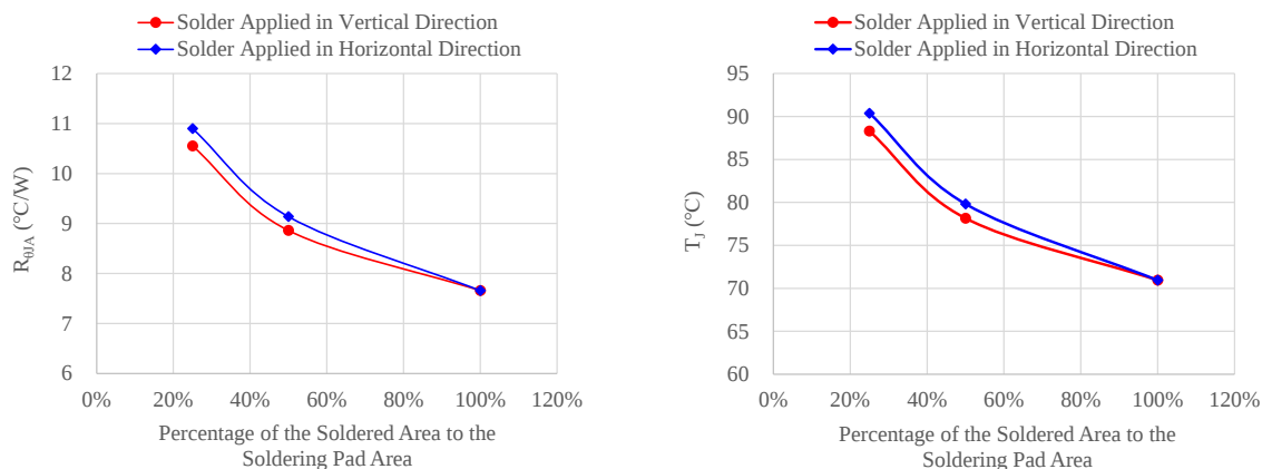
Figure 12. The R_{\theta JA} and T_J Values Measured with Different Amounts of Solder Paste
