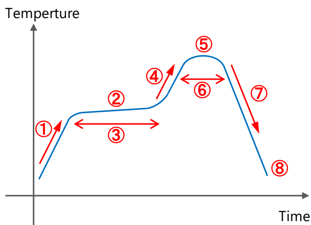
Figure 25. Description of where the reflow conditions are adjusted
