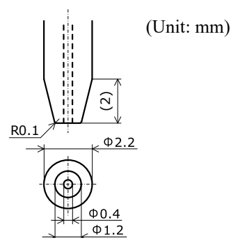
Figure 13. Recommended Nozzle
